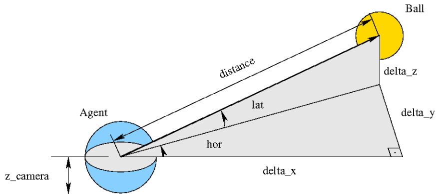
Figure 4.3: Polar coordinates as supplied by the 3D Soccer Server [Vor06]
